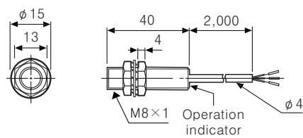
●PRL08-2D□
