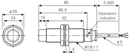
●PRL18-8D□
