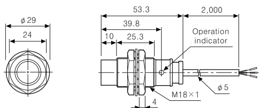
●PR18-8A□
