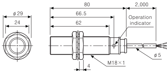
●PRL18-8D□
